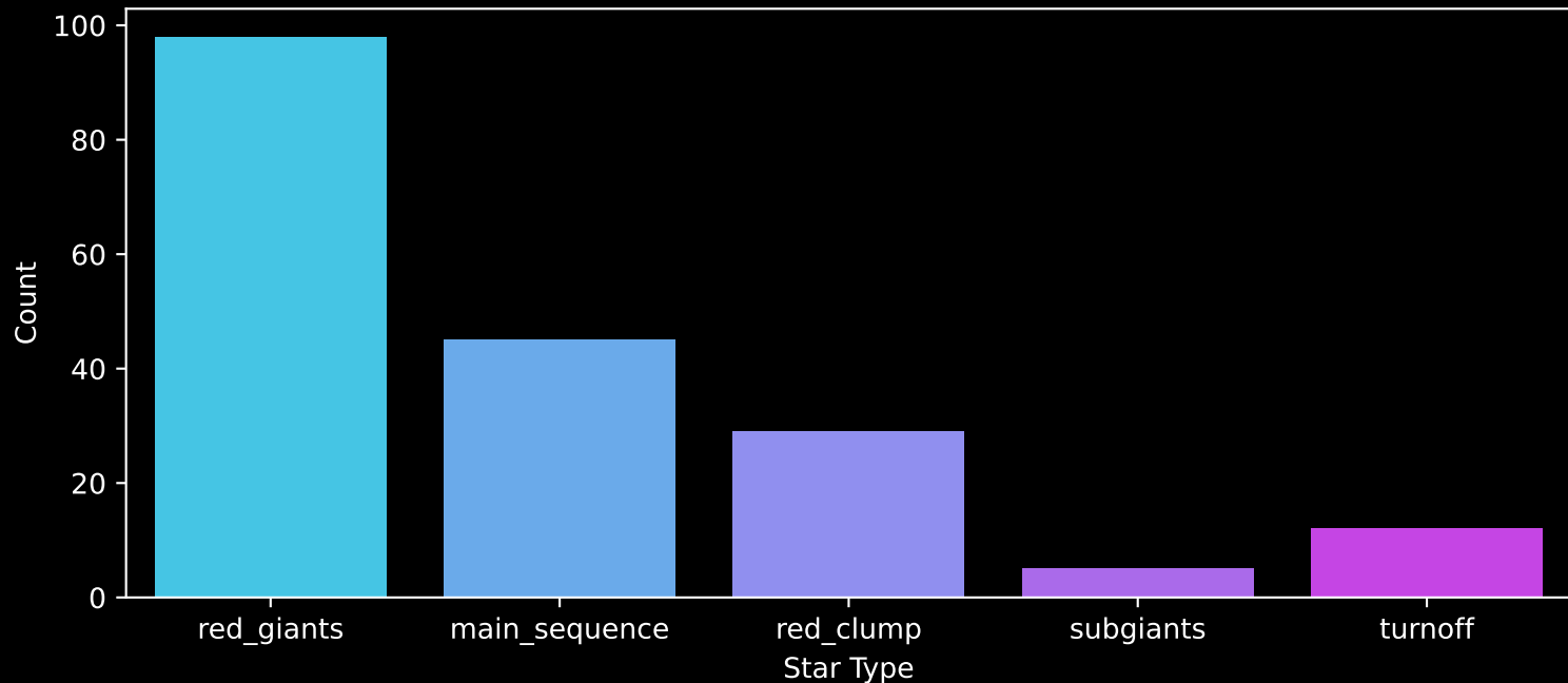
APOGEE DR17 Field: [195+30_MGA] Count plot of Star Type
