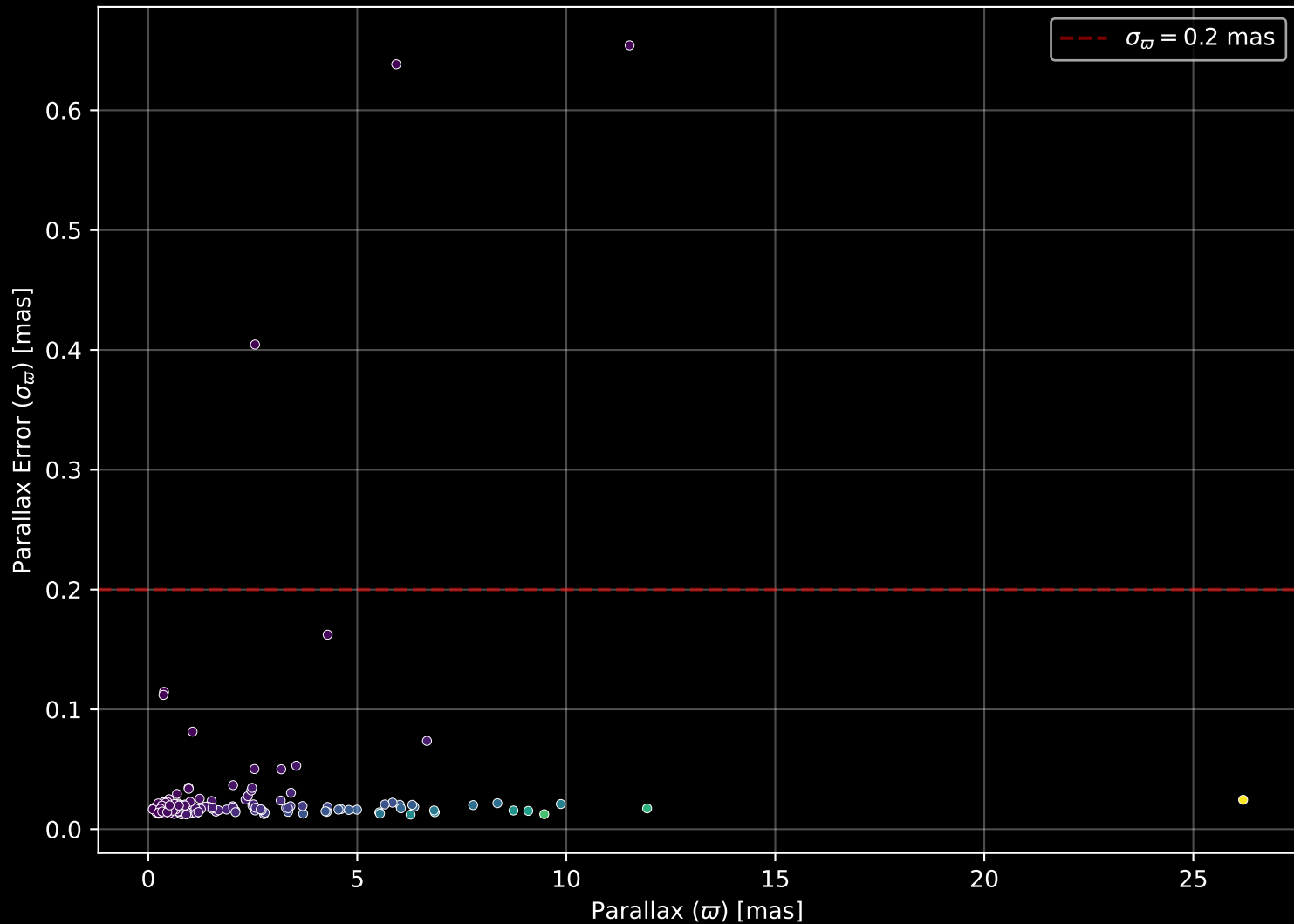
APOGEE DR17 Field: [195+30_MGA] Parallax Quality (n= 189)
