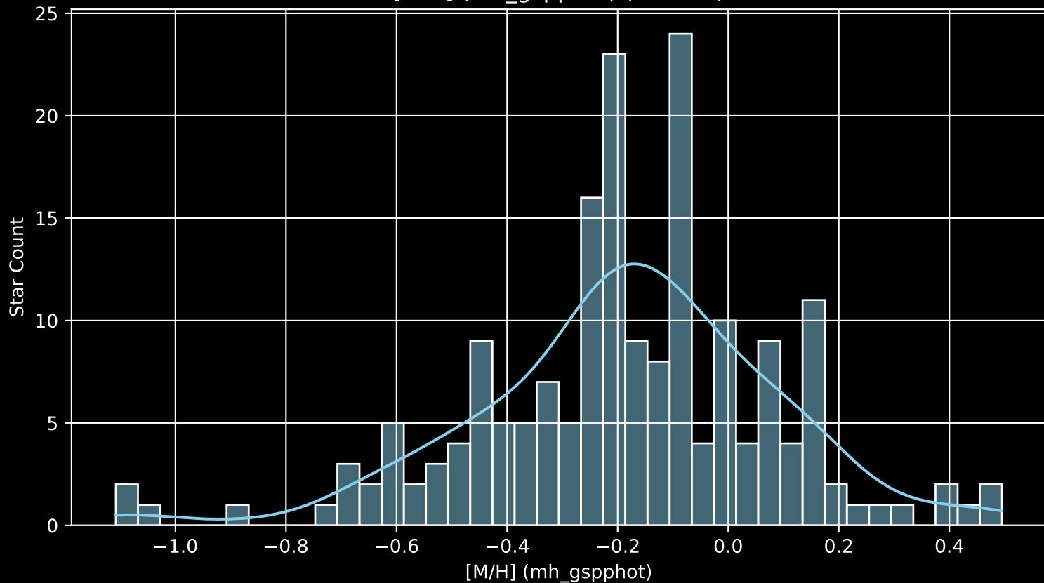
APOGEE DR17 Field: [195+30_MGA [M/H] (mh_gspphot) (n= 187)
