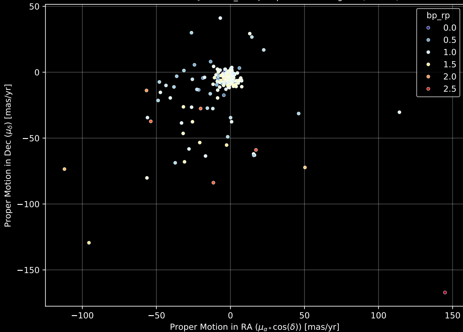
APOGEE DR17 Field: [195+30_MGA] Proper Motion Diagram (n= 189)
