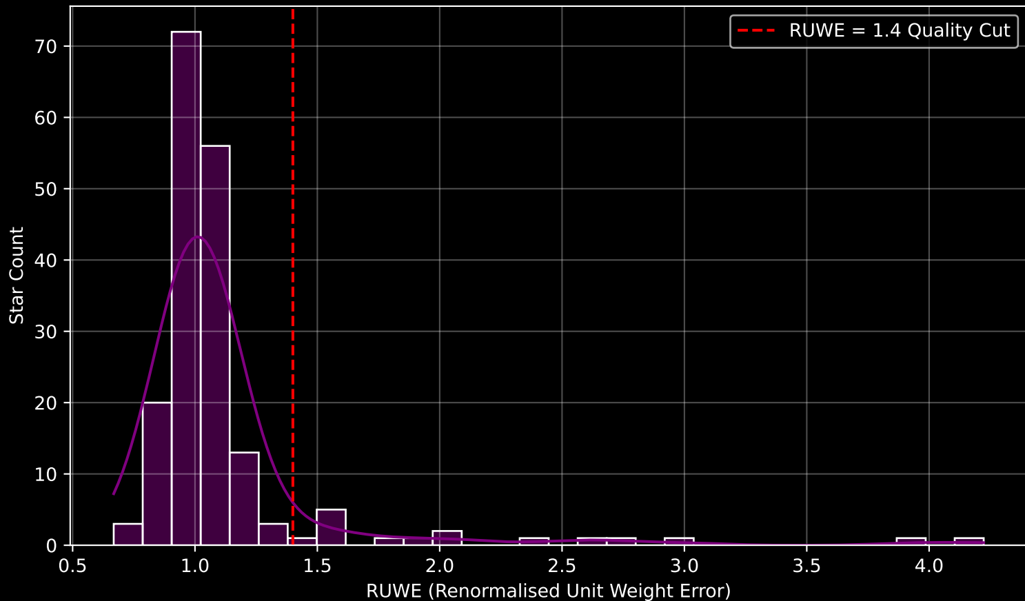
GAPOGEE DR17 Field [195+30_MGA] RUWE Distribution (n= 183)
