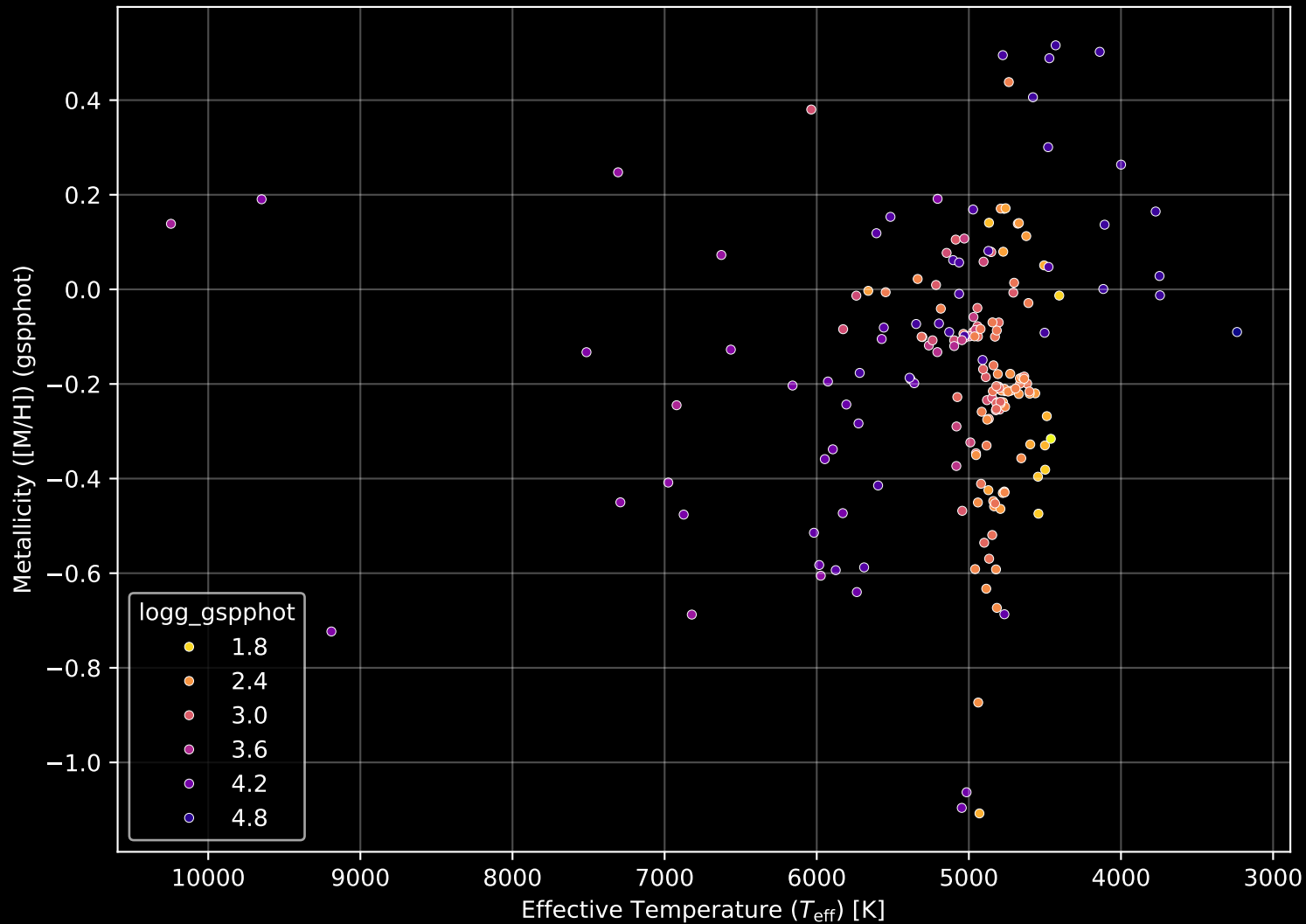
APOGEE DR17 Field: [195+30_MGA] Stellar Population Parameters (n= 189)
